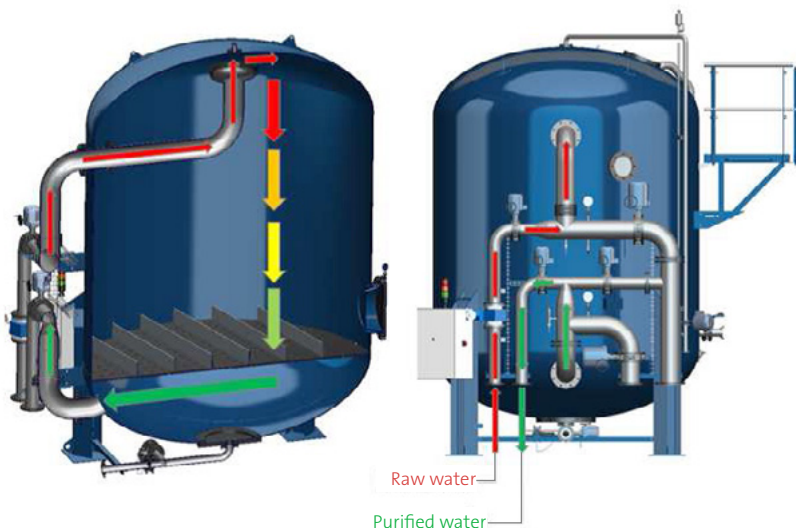
FILTRAFLO PACK (Mono/Duo/Trio) water filtration process
